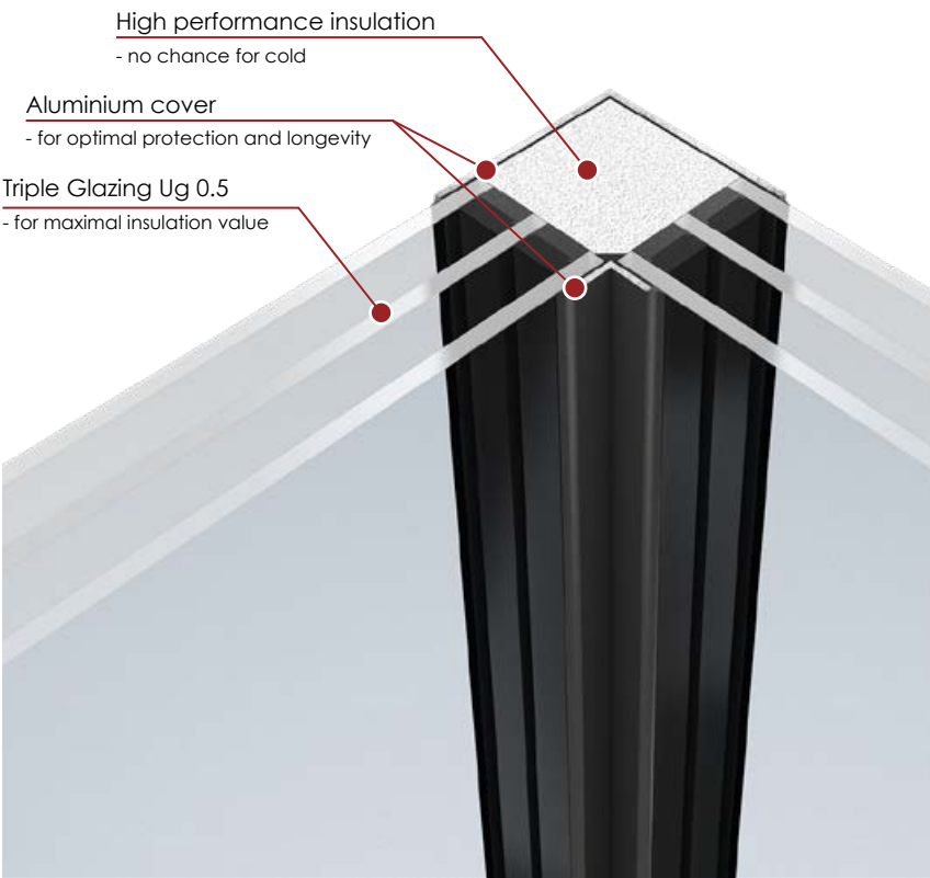
Insulated glass corner streamlined insulating capacity and durability
